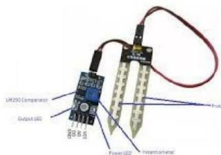
Fig. 3: Soil moisture sensor
